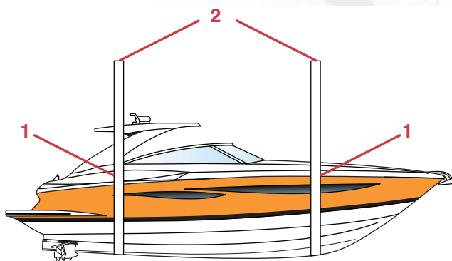
1 – Sling Tag Location 2 – Flat, Wide-belted Sling
