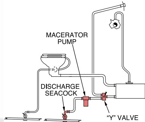
TYPICAL MACERATOR SYSTEM
